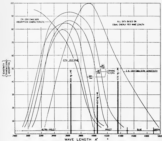
FIG. 1. Sensitivity and absorption curves of sound negative emulsion and transmission characteristics of filters. Based on equal energy per wavelength.
